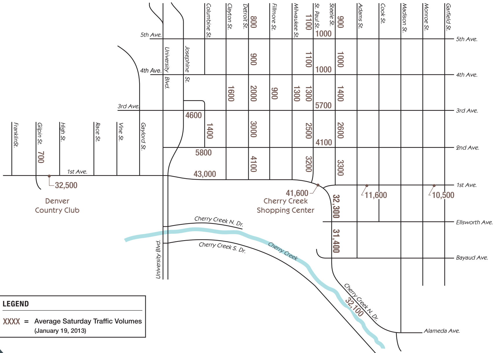
Figure 3 Existing Saturday Traffic Volumes
